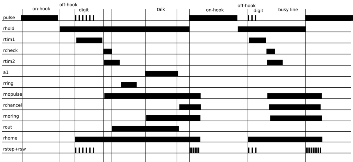
Figure 10: Second Timing Diagram
