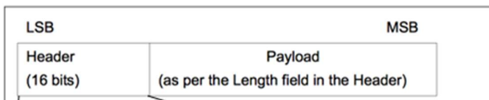
Figure 2.2: Advertising channel PDU
