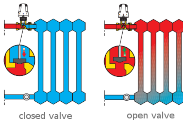
Fig. 2: Operating scheme of a classic valve 1
