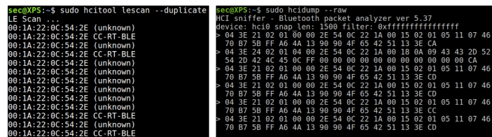
Fig. 28: Hcidump ( right ) running while scanning ( left )
