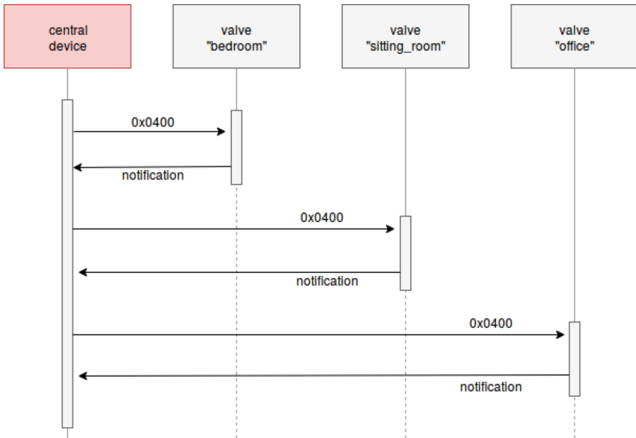
Fig. 31: Sequence Diagram of auto_mode.sh
