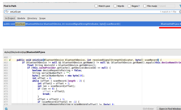
Fig. 20: Android Studio “Find in path” window
