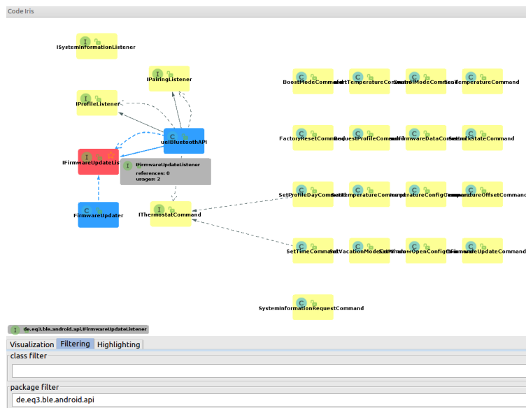
Fig. 22: Class View with Filtering Enabled
