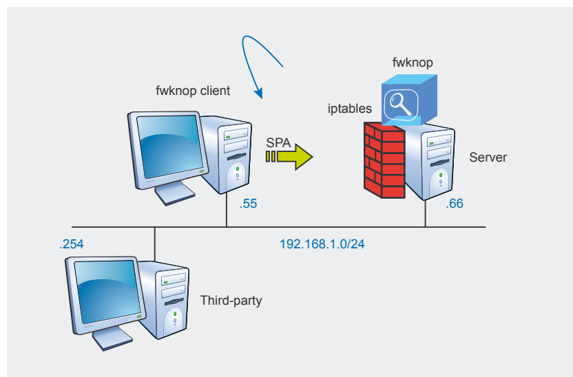
Figure 1. Basic port knocking architecture
