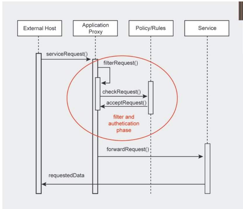
Figure 3. Sequence diagram that shows how an external host request is filtered, checked and, if allowed, finally accepted
