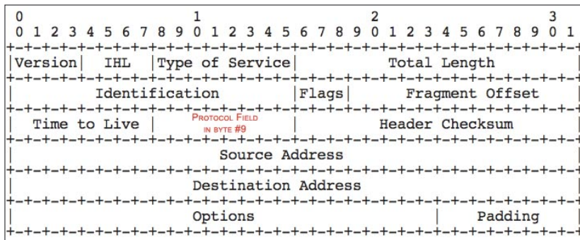
Figure 1. IP protocol header, note that one tick mark represents one bit position
