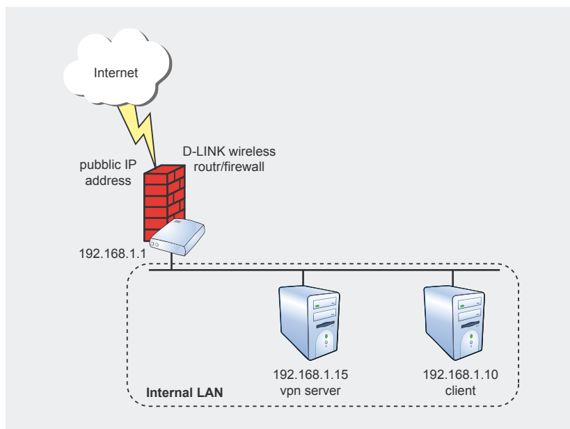
Figure 3. Typical home DSL network
