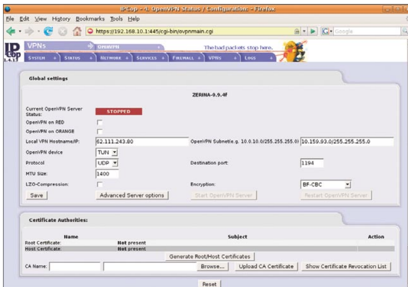
Figure 5. OpenVPN
