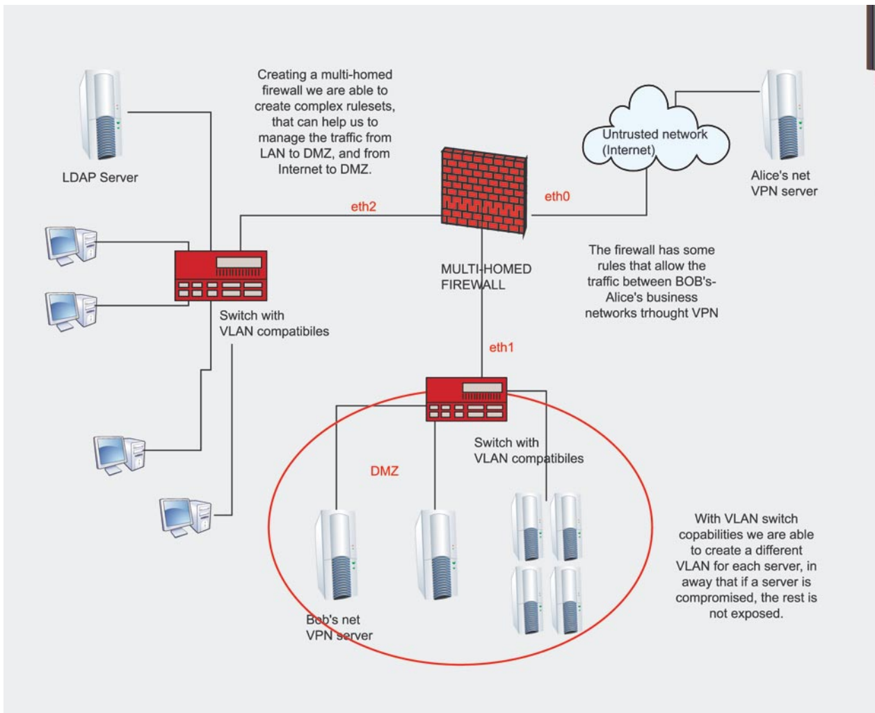
Figure 5. A multi-homed firewall that manage a LAN and a DMZ, and their connection with the a trusted/untrusted network (in this case the Alice NET as trusted – thought a VPN – and Internet as untrusted)
