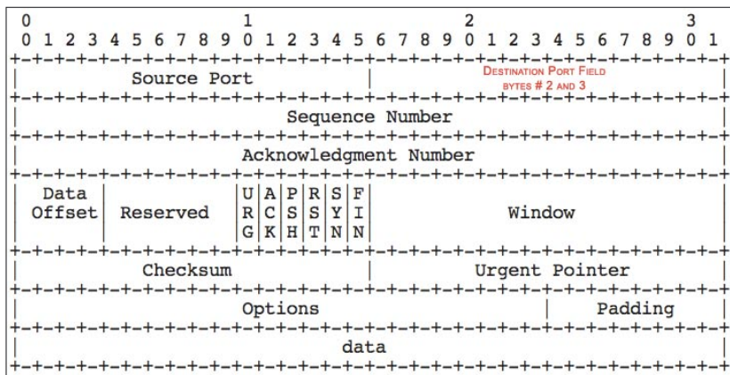
Figure 2. TCP protocol header, note that one tick mark represents one bit position
