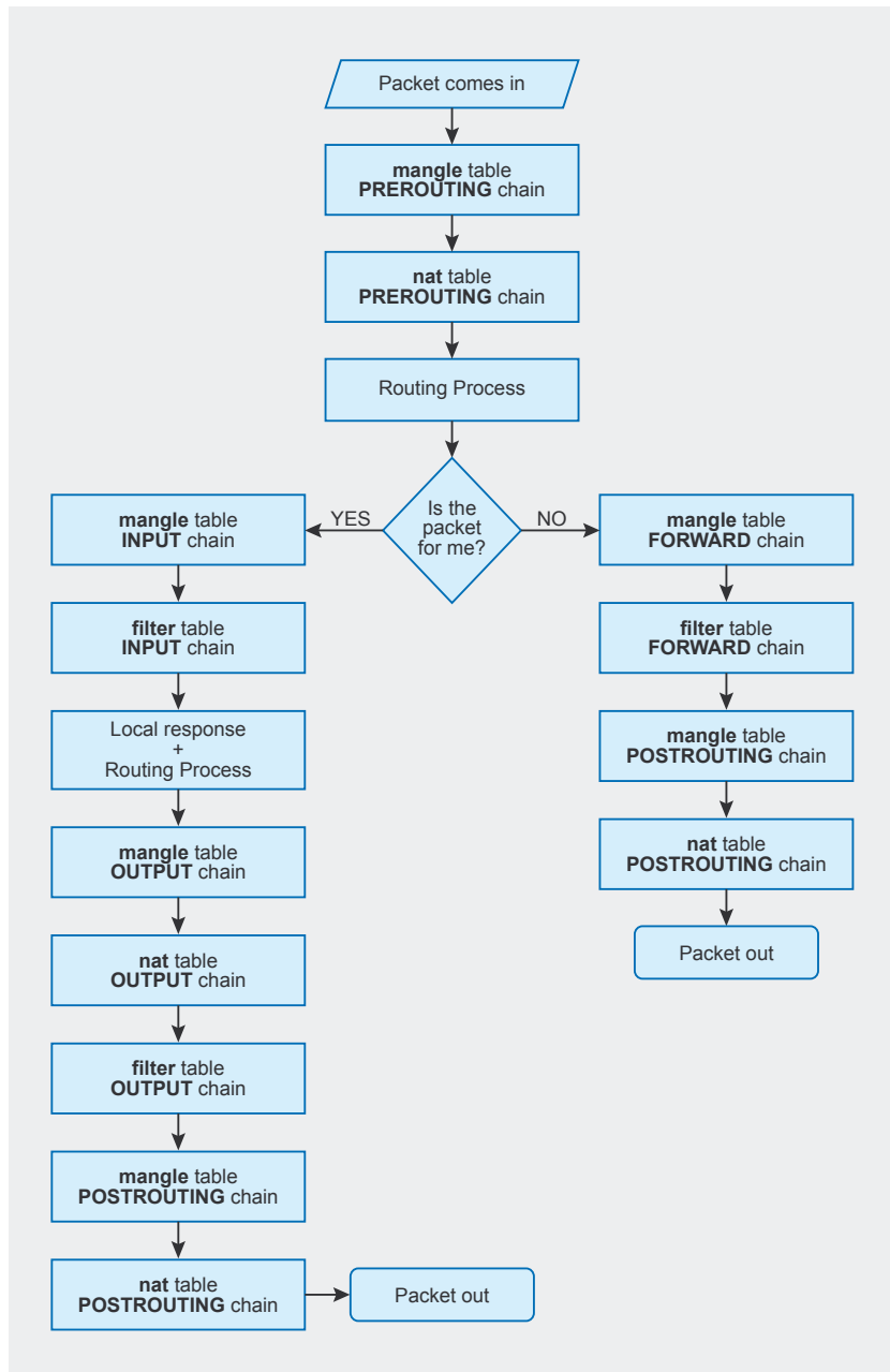
Figure 1. Filtering rules in five chains
