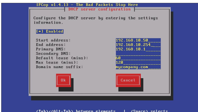
Figure 2. DHCP configuration
