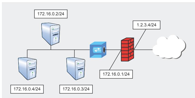
Figure 1. In-and-Out
