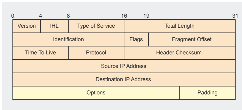
Figure 2. The header of all IP packets
