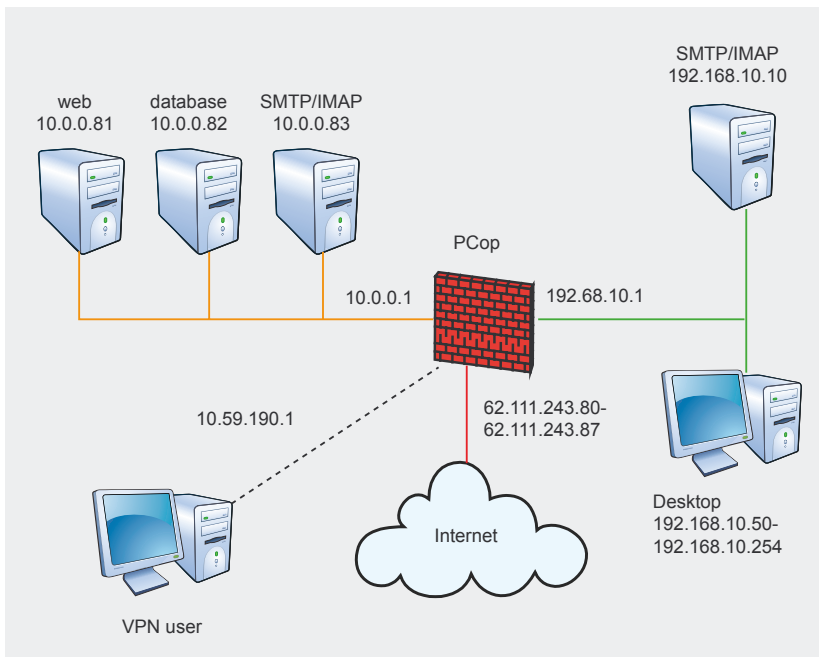
Figure 1. Company network
