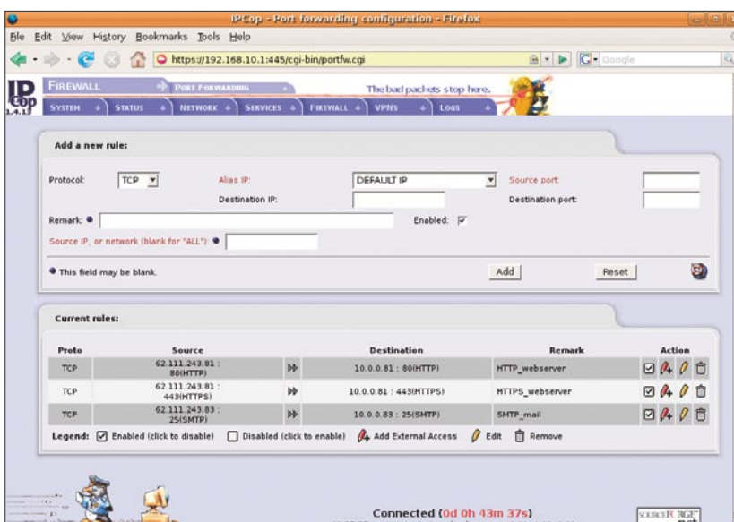
Figure 4. Port forwarding
