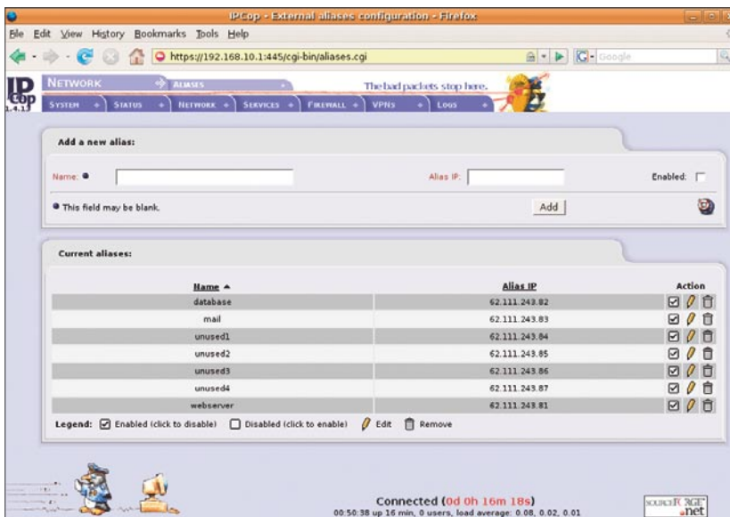
Figure 3. Aliases
