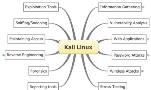
Figure 2. Directory Structure
