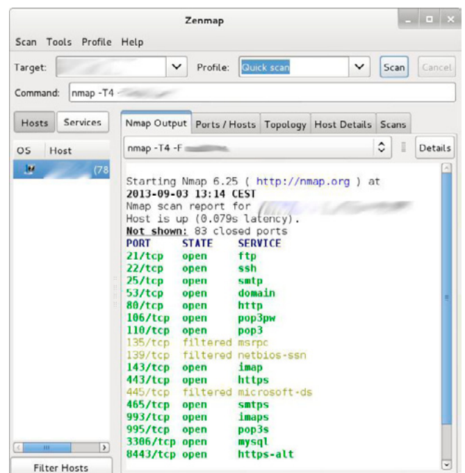
Figure 1. Result of scan with Zenmap. Multiples open ports
