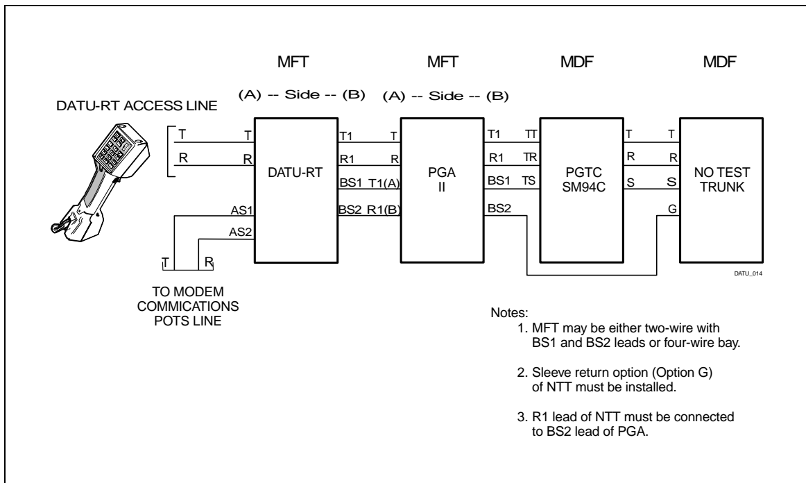
Figure 2-3. Connections for All Systems Except 5 ESS with Integrated SLC Only, DMS-10 and DMS-100
