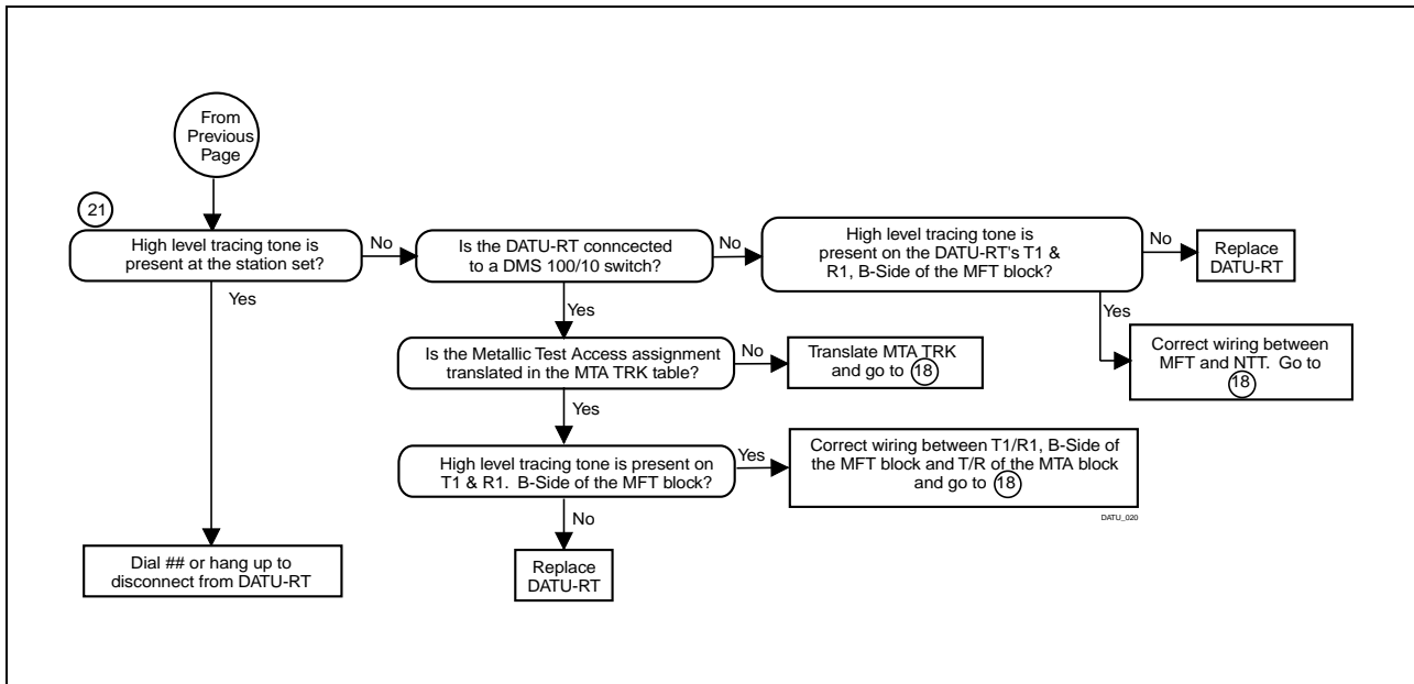
Figure 5-1. Fault Location Flow Chart (Sheet 6 of 6)
