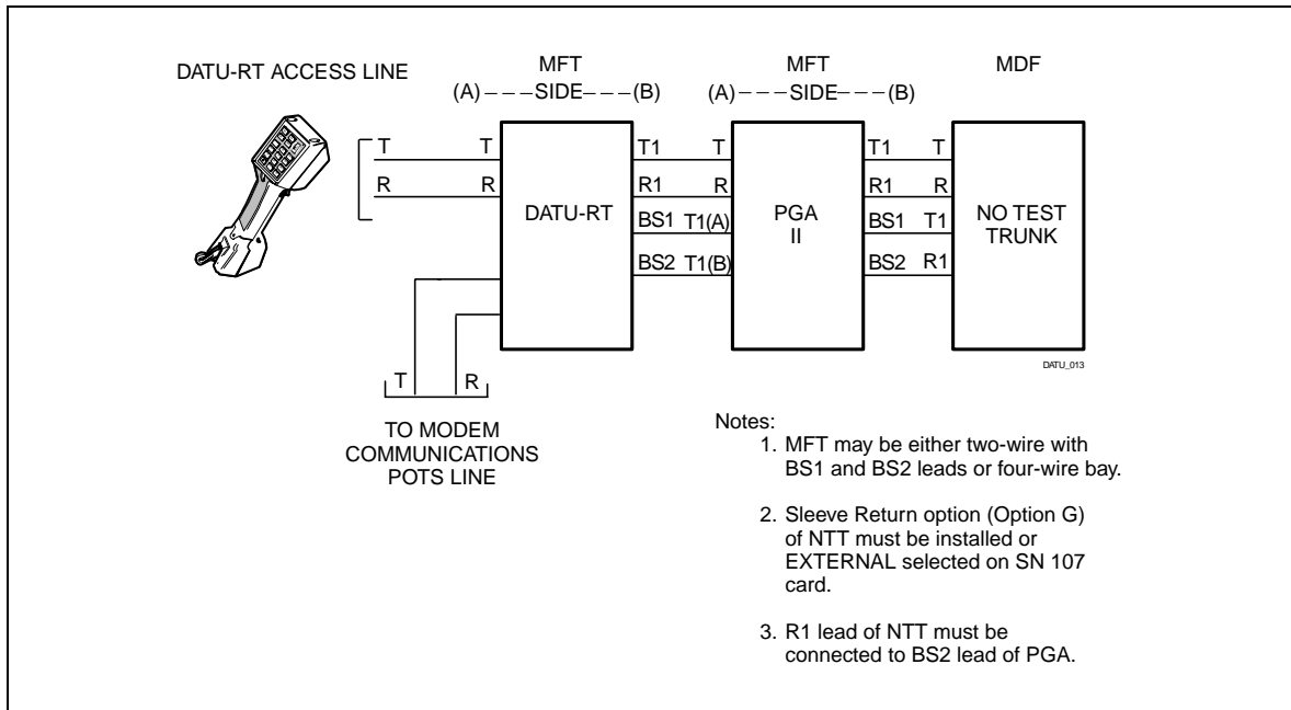
Figure 2-4. System Connections for 5 ESS with Integrated SLCs Only
