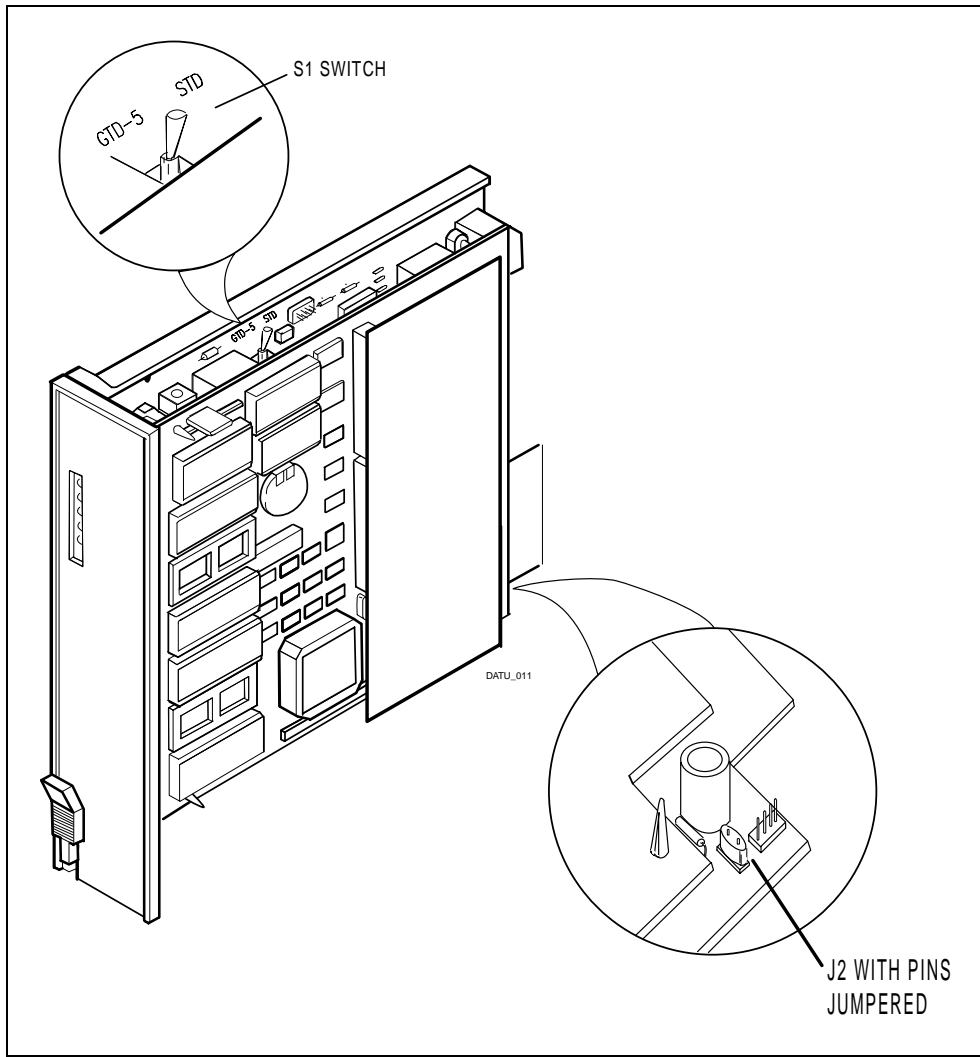
Figure 2-2. DATU-RT J2 and S1 Switch Locations
