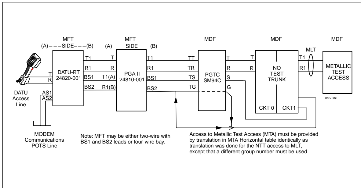
Figure 2-5. DMS-100 MDF Connections
