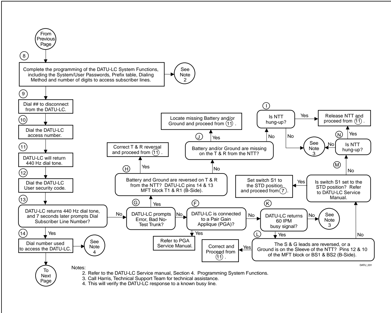
Figure 5-1. Fault Location Flow Chart (Sheet 3 of 6)
