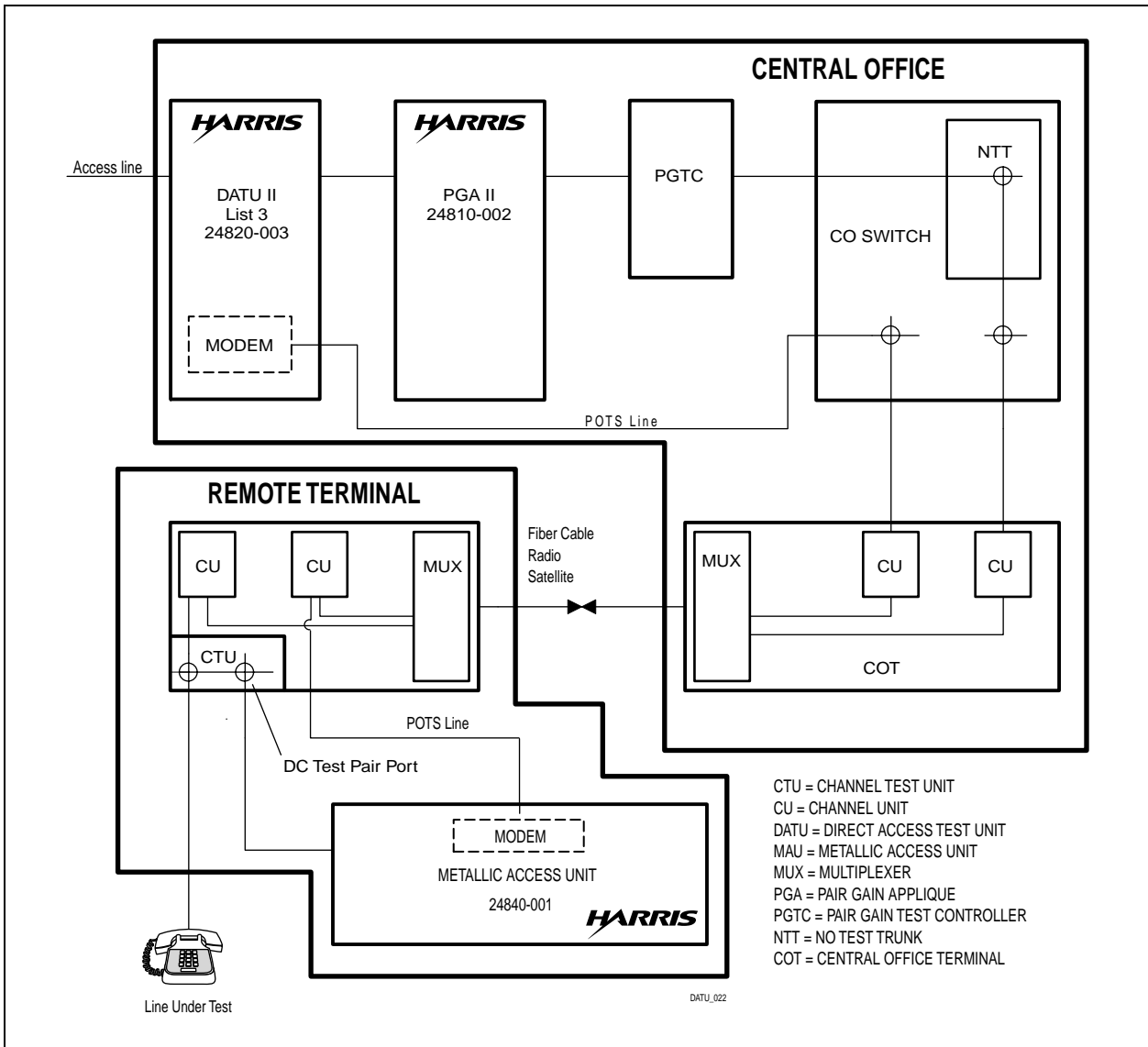
Figure 1-1. DATU-RT System Application Diagram
