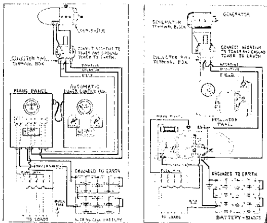
Two different wire systems used by Win barge
