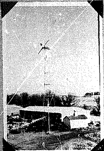
PHOTO 14. Air Electric 2000 Watt - 32 Volt - On Tower
