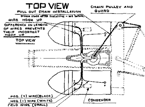
FIGURE B Jacobs Twin-Motor 1500 Watt - 32 Volt - Model 15
