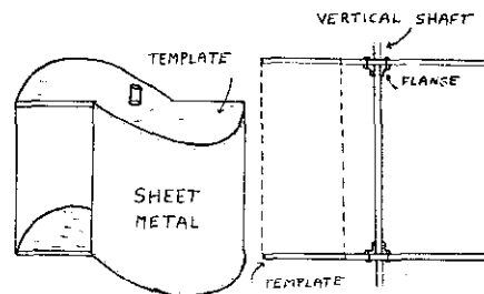
Figure 4 Savonius Wing Assembly.
