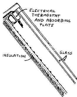
Figure 4 Position of thermostat in solar collector.
