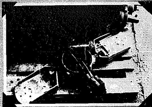
PHOTO 4. Wincharger Governor
