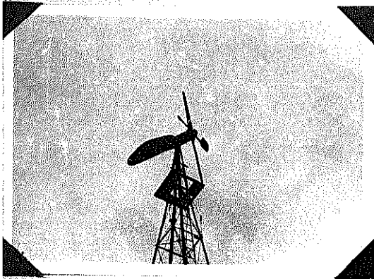
PHOTO 17 Air Electric 3000 Watt - 32 Volt - Paddle type Governor
