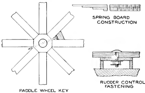
Detail of Paddle-Wheel Fastening, the Springboard Construction and the Fastening for the Rudder Control
