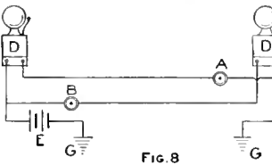
Wiring Diagrams for Return-Call Bells
