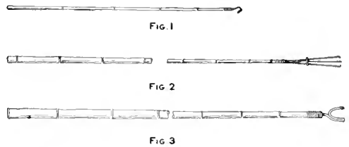
A Bamboo Pole Cut in Three Pieces Makes a Window Shade Stick, Duster Holder and Clothesline Pole
