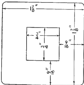
Fig. 14—Insulating Washer
