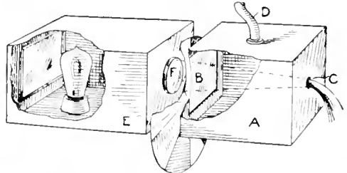
The Arrangement of the Boxes Showing the Path of the Light Rays through the Water
