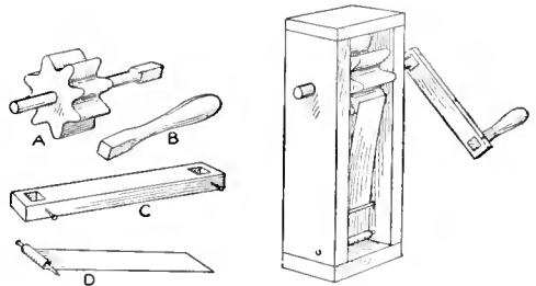
Detail of the Parts and How They are Assembled to Make the Clapper
