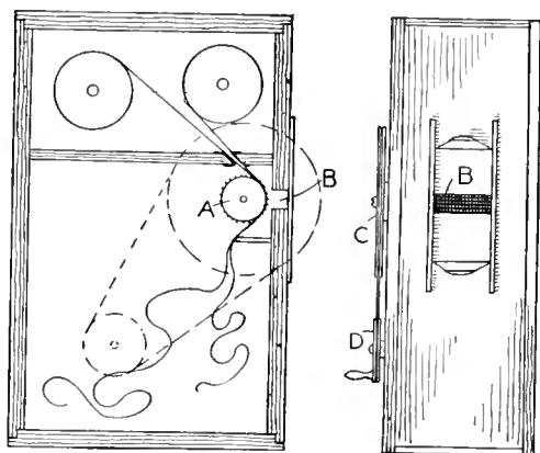
Fig. 7—Printing Machine
