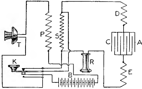
Fig. 7—Sending and Receiving Equipment
