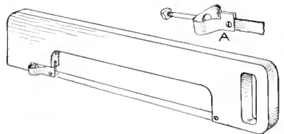
Hacksaw Frame, Cut from Hard Wood, with Fittings Attached to Draw the Blade Taut
