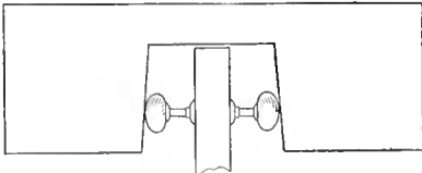
The Sloping Edges in the Notch Forces the Knobs Together and Holds Them While Inserting the Screws
