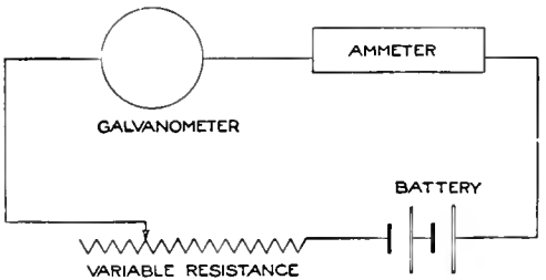
FIG. 4 The Electric Circuit, Showing Connections for Finding the Value of a Current in Calibrating
