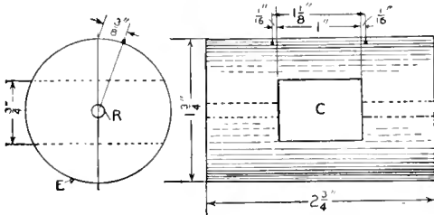
Fig. 3—Details of Shutter
