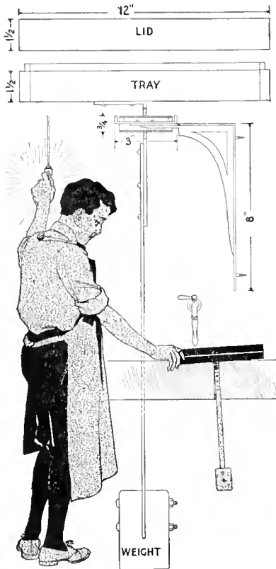
Developing-Tray Rocker to Keep the Liquid in Motion over the Plate Automatically
