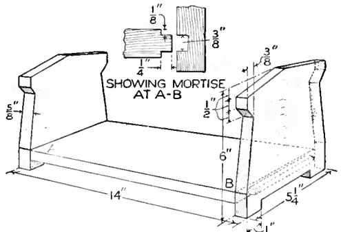
A Bookrack That can be Made in Any Wood to Match Other Furniture
