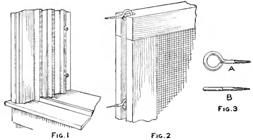
The Heads of the Screweyes in the Window-Frame Stop Slide in a Groove Cut in the Screen Frame
