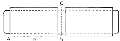
A Wood Mandrel Used to Face the Ends and Turn Flanges on Tubing for Cylinders
