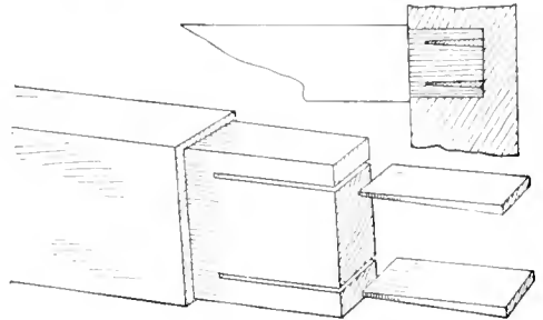
Wedges in Tenon
