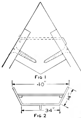
The Skiff is Especially Constructed for Use in Shallow Water and Marshes by Duck Hunters, but with the Addition of a Keel It Makes a Good Craft for Almost Any Water as a Rowboat
