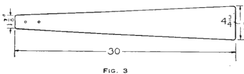
The Hub Consists of Two Parts, Each Having Four Arms for Holding the Blades
