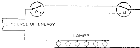
FIG. 1 Lamps Controlled from Two Switches
