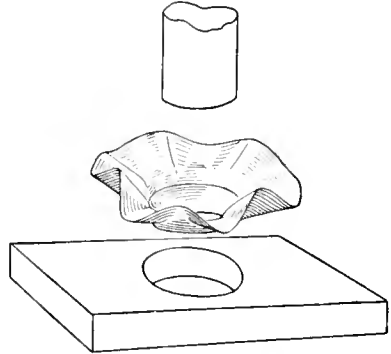
The Former and Method of Using It to Produce a Wrinkled Edge on the Tray
