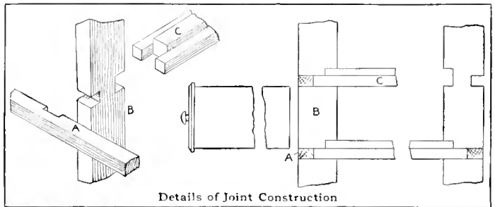
Details of Joint Construction
