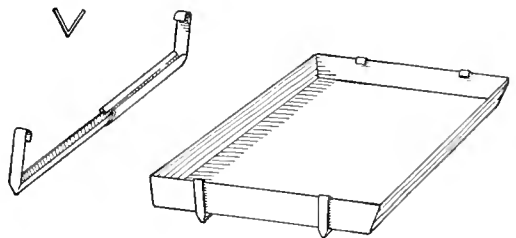
Shoe and How It is Attached to the Pan
