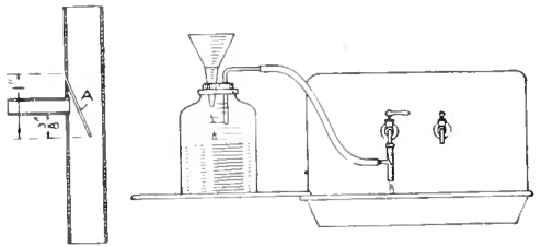
Detail of the Aspirator and Its Connections to a Faucet, for Increasing the Speed of Filtration
