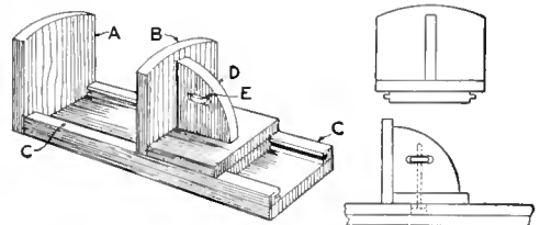
The Holder may be Used for Books or Letters and Papers as a File
