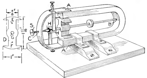
Detail of Armature Laminations, and Completed Parts Assembled, but without Armature Windings
