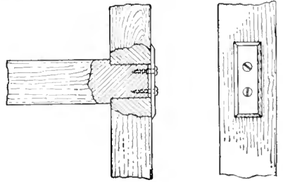
Metal Covering and Holder for a Tenon and Mortise Joint on Mission Furniture
