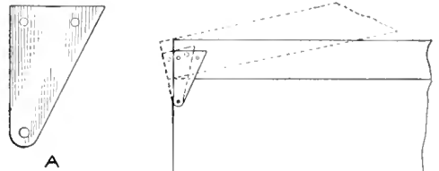
Hinge Parts Made of Sheet Metal and Their Use on a Box Cover
