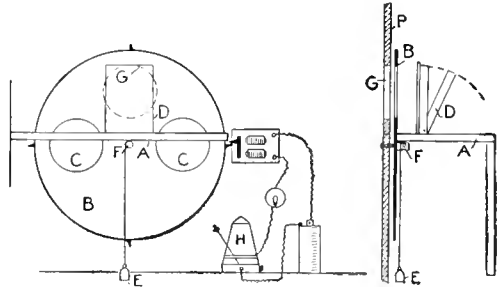
Details of Timing Apparatus
