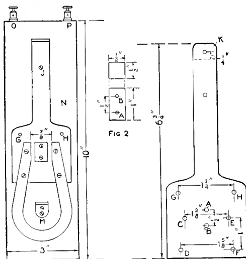
FIG. 1 The Permanent Magnet and Its Brass Support, and Their Position on the Base
