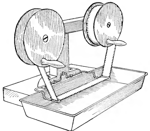
Fig. 5—Developing Long Films
