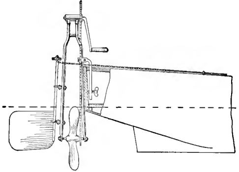
The Rear Fork of a Bicycle with Its P. rts Constitutes the Main Propeller Attachment
