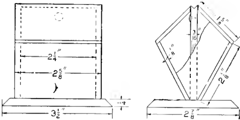
The Box Delivers Only One Match When It is Raised and Lowered on the Standard
