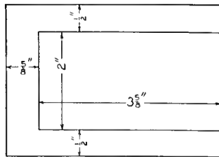
Fig. 12 — Outer Portion of the Magnetic Circuit
