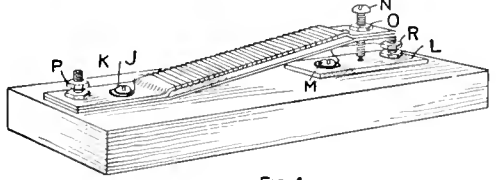
FIG. 4 The Assembled Parts Showing the Complete Flasher and Electric Connections with Adjusting Screw
