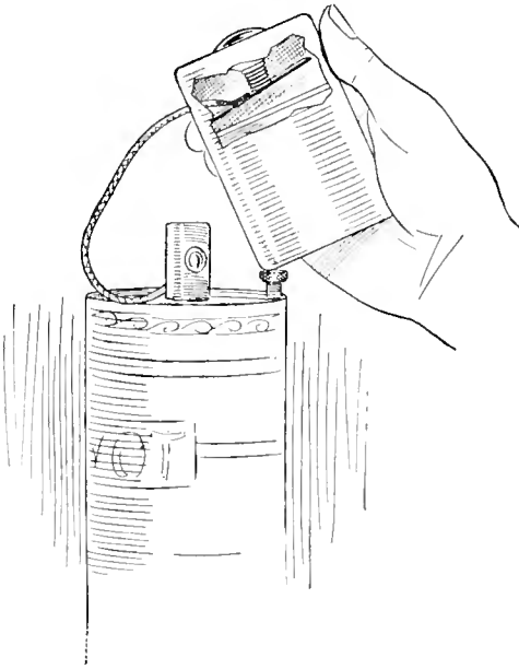
An Instrument Made of an Electrical Pocket Flash Light for Testing Circuits and Instruments
