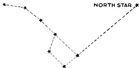
The Two Stars at the End of the Great Dipper are Pointers to the North Star
