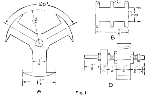
Fig. 1 Details of the Armature Laminations and the Commutator Segments, and the Method of Mounting Armature Core and Commutator
