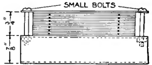
Fig. 19—Method of Clamping Transformer Together
