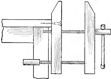
The Clamp Attached to a Bench Top will Serve the Purpose of a Vice in Many Instances
