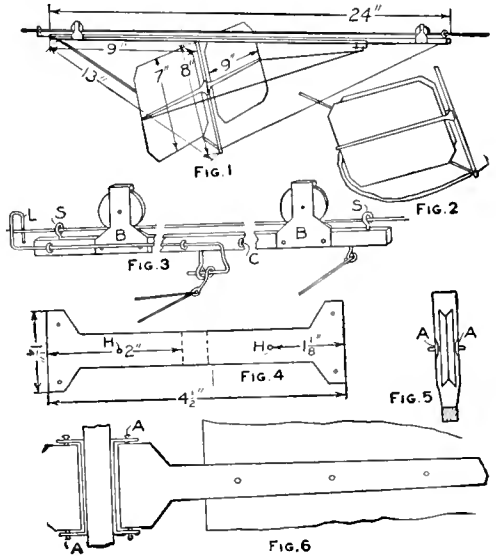
Traveler Details
