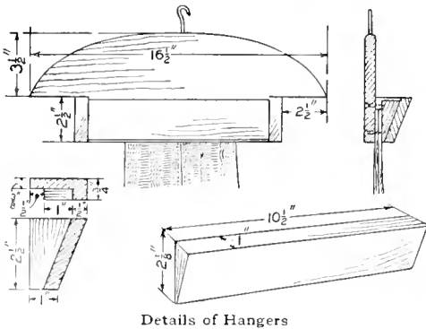
Details of Hangers
