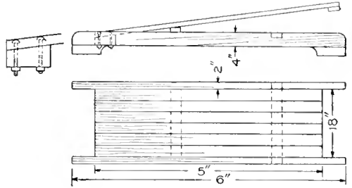
A Springboard for Use in Connection with a Vaulting Pole or for Turning Acts
