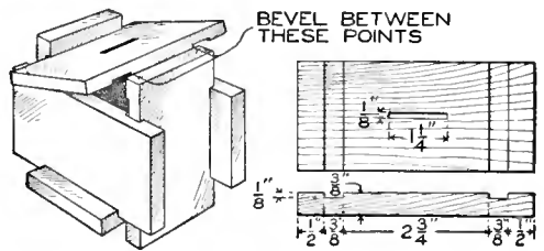
Six Pieces of Wood as They are Put Together to Form a Toy Bank
