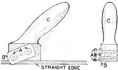
FIG. 2 Blade Attached to Handle
