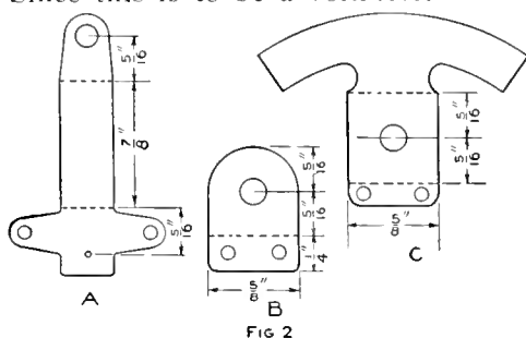
FIG 2 Details of the Supports for the Coil and for the Needle, or Pointer, Shaft
