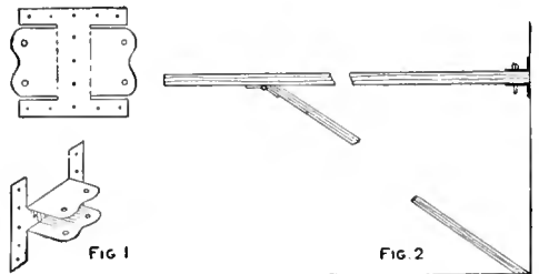
FIG. 1 FIG. 2 Socket and Manner of Holding Board
