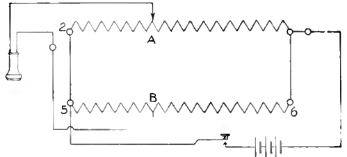
Fig. 1—The Diagram of a Wheatstone Bridge Which Shows the Points of Contact So Placed That a Balance is Obtained
