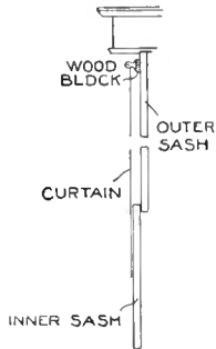
When the Upper Sash is Lowered the Shade is Out of the Way of the Opening
