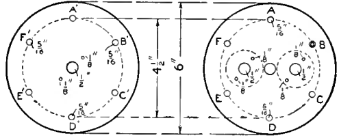
FIG. 1 FIG. 2 Detail of the Two Ends on the Heater Giving Dimensions and the Location of Parts
