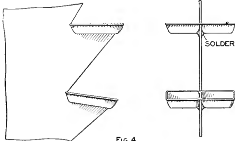
The Water Cups are Fastened to the Teeth on the Metal Disk with Solder
