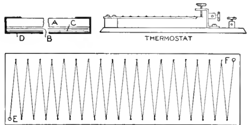
Fig. 2—Heater Details
