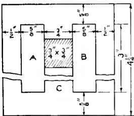
Fig. 11 — Complete Magnetic Circuit
