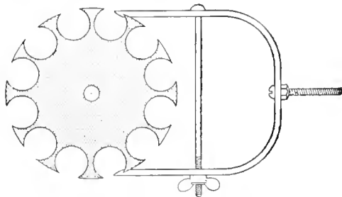
Armature Cores are Easily Revolved to Fill the Core Openings with Insulated Wire
