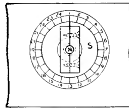
The Parts as They are Attached to a Drawer Front to Make a Combination Lock
