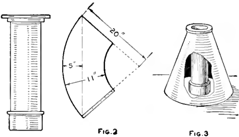
FIG. 1 The Parts to Make the Crucible Consist of Pipe and Fittings and a Piece of Sheet Metal
