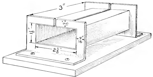
Dimensioned Parts for the Construction of the Core over Which the Insulated Wire is Wound
