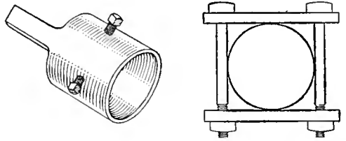
Two Forms of Lathe Dogs That are Quickly and Cheaply Constructed
