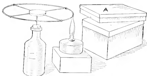
The Wheel as It is Mounted on a Needle, and Lamp and Box Containing Magnet to Make It Turn
