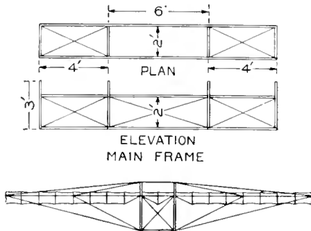
Details of Tandem Monoplane Glider, Showing the Main Frame and Wing Construction, and the Manner of Placing the Crossed Bracing Wires Between the Parts and to the Wing Ends
