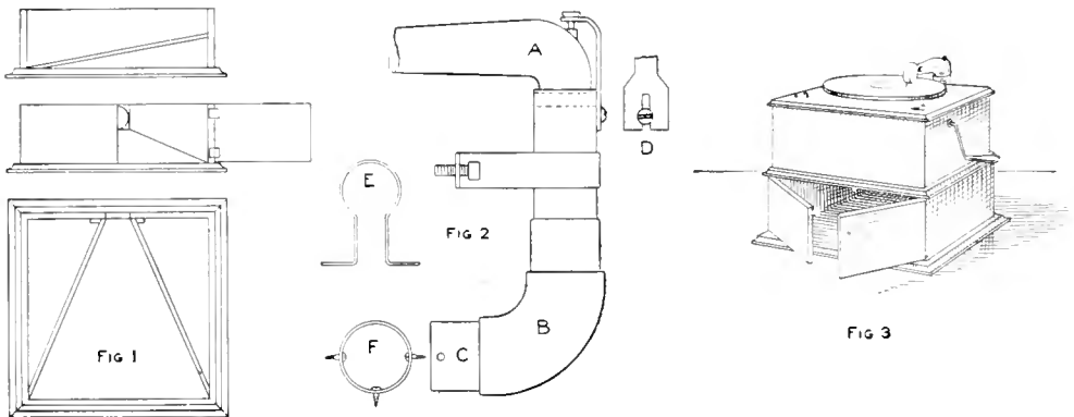
The Horn or Sounding Box is Constructed in the Auxiliary Base and the Part for Connecting the Sounding Tube to the Box Consists of Ordinary Gas Pipe Fastened with a Clip at the Back
