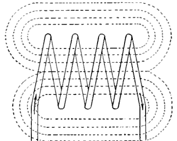
Fig. 6—A Coil about a Magnetic Circuit through Iron and Air
