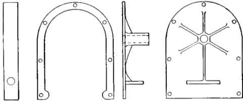
FIG. 4 Metal Casing Instead of Wood
