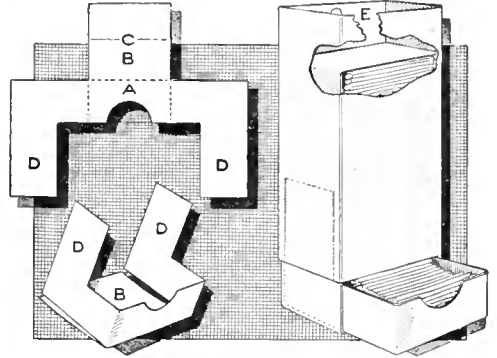
The Attachment Consists of a Receptacle Fitting into the End of a Match Box
