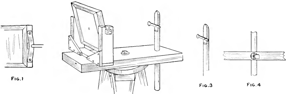
FIG. 1 FIG. 2 FIG. 3 FIG. 4 Detail of the Parts for Making the Mirror and Sight Rod Which are Placed on a Base Set on a Tripod Top, the Whole being Adjusted to Reflect the Sun's Rays in Any Direction Desired
