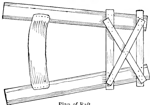
Plan of Raft
