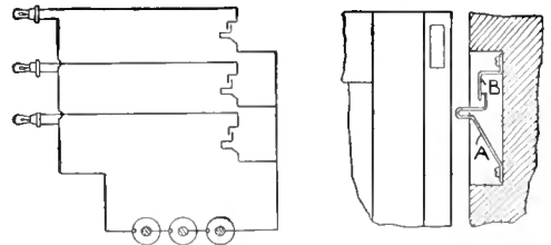
FIG. 1 The Lamps will be Automatically Lighted When the Door of the Ice Box is Opened
