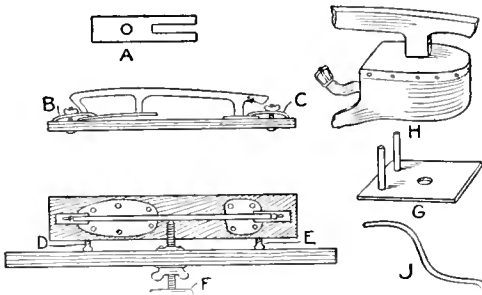
The Holder Provides a Way to Grind a Slight Curve in the Edge of a Skate Blade
