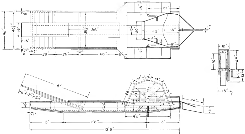
Detail Drawing of the Boat and One of the Paddle Wheels. All the Material Required for the Construction is Such That can be Cut and Shaped with Ordinary Tools Found in the Home Workshop
