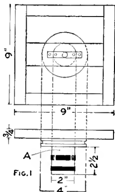
Details of the Different Parts to Construct the Electric Fountain
