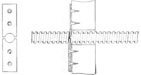
Two Pieces of Strap Iron Shaped to Fit the Square Thread Make a Good Substitute Nut
