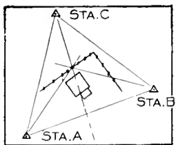
Three Stations are Used for Setting the Plane Table in Succession to Locate the Various Objects
