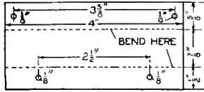
Fig. 17—Lower Clamping Pieces and Mounting Supports
