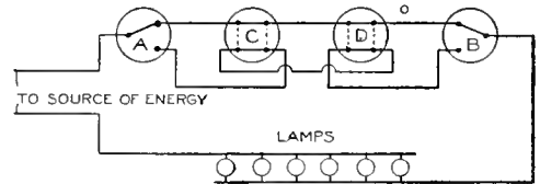
FIG. 2 Lamps Controlled by Any Number of Switches
