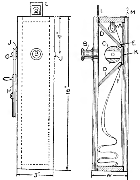
Fig. 2—Details of Camera
