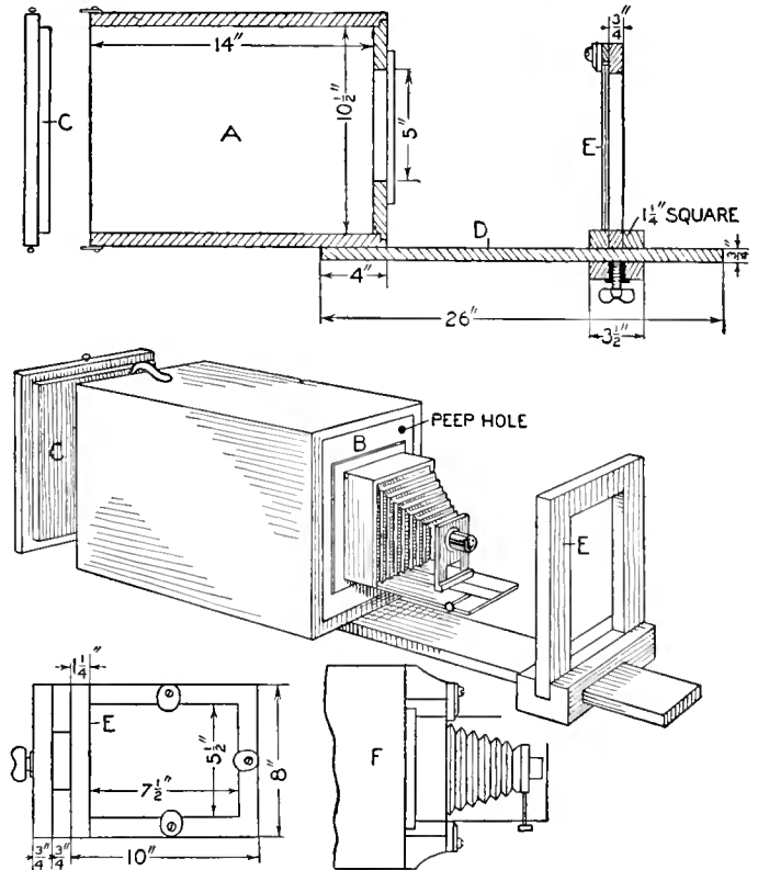
Details of Construction and Camera Complete
