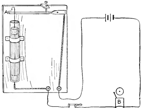
The Alarm and Wiring Diagram
