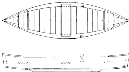
The Skiff is Especially Constructed for Use in Shallow Water and Marshes by Duck Hunters, but with the Addition of a Keel It Makes a Good Craft for Almost Any Water as a Rowboat
