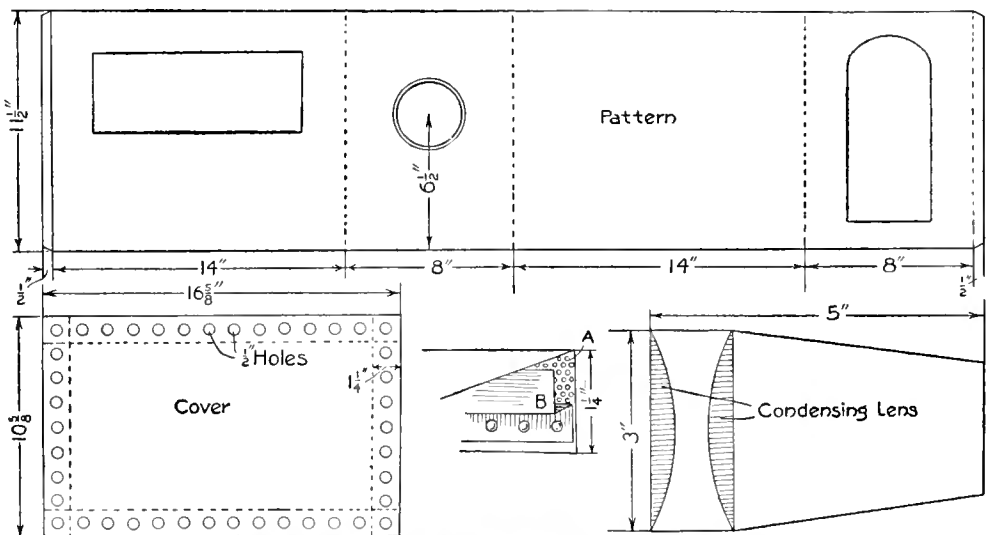
Fig. 9 — Details of the Lamp House
