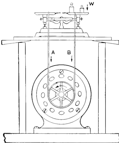
Prony Brake Used in Connection with a Small Balance to Find the Horsepower
