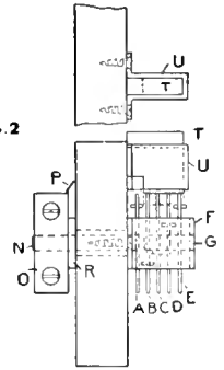
The Parts as They are Attached to a Drawer Front to Make a Combination Lock
