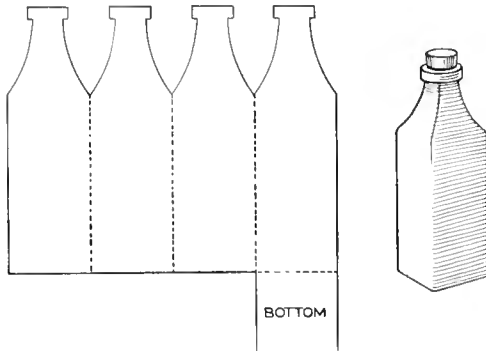
Pattern for Making a Bottle Cover of Leather or Rubber for Bottles Carried in the Pocket
