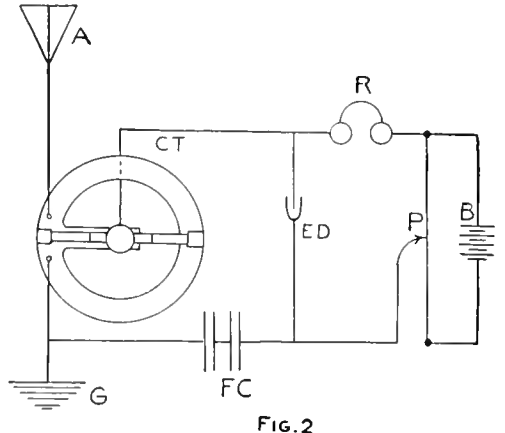
Tuning Coil and Wiring Diagram
