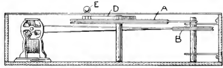
The Steel Ball is Caused to Roll Around on the Cover by the Moving Magnet
