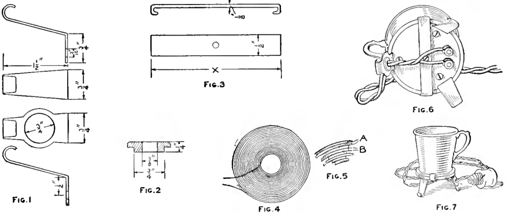
Detail of the Parts for the Construction of an Electric Shaving Mug. The Heating of Sufficient Water for a Shave can be Accomplished at a Nominal Cost
