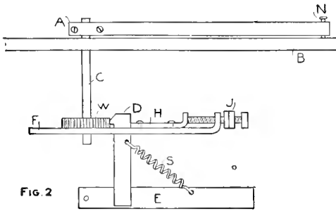
Details of Gear-Cutting Machine
