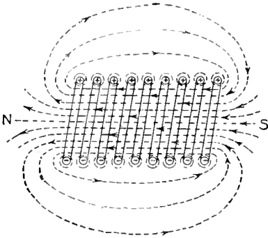
Fig. 5—Magnetic Lines Passing through Center
