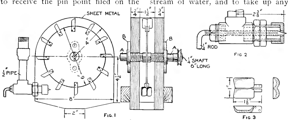
FIG. 1 Details of the Water Wheel
