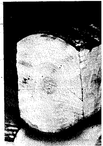
PLATE 63 The two sides hewed, the log is now ready for notching. The remainder of the sides will be hewed after the logs are all in place in the cabin.
