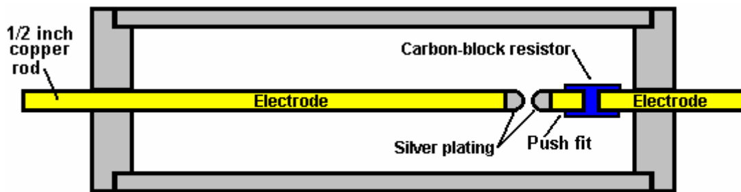
VIEW SHOWING THE ELECTRODES IN PLACE
