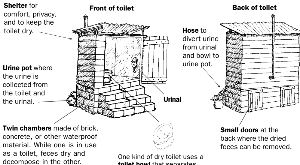
Parts of the twin chamber dry toilet
