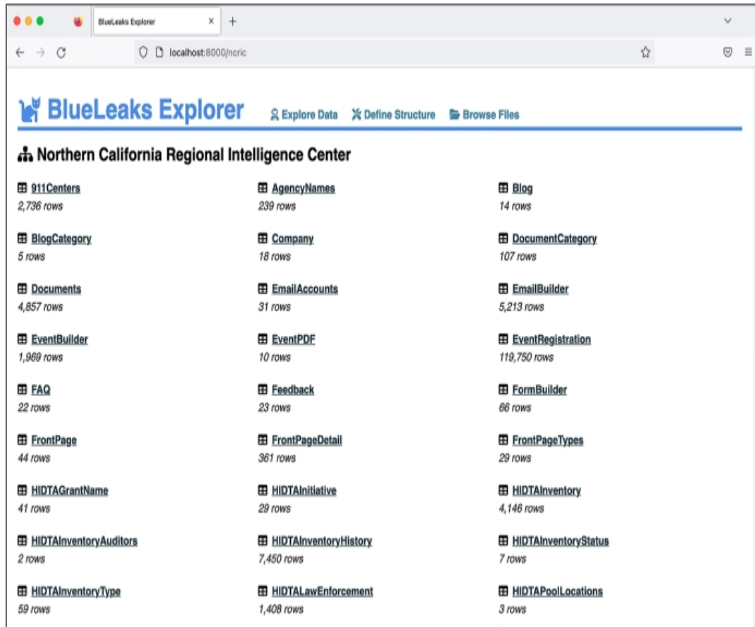
Figure 10-2: Viewing the NCRIC tables in BlueLeaks Explorer
