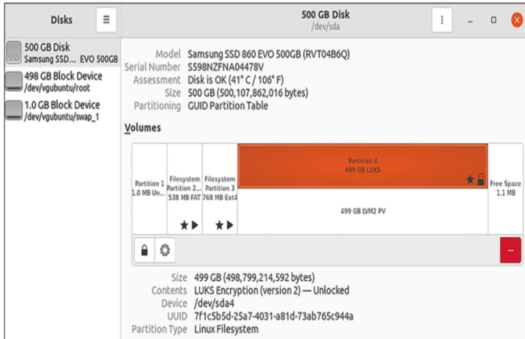
Figure 1-3: Managing disks and partitions using Disks in Linux
