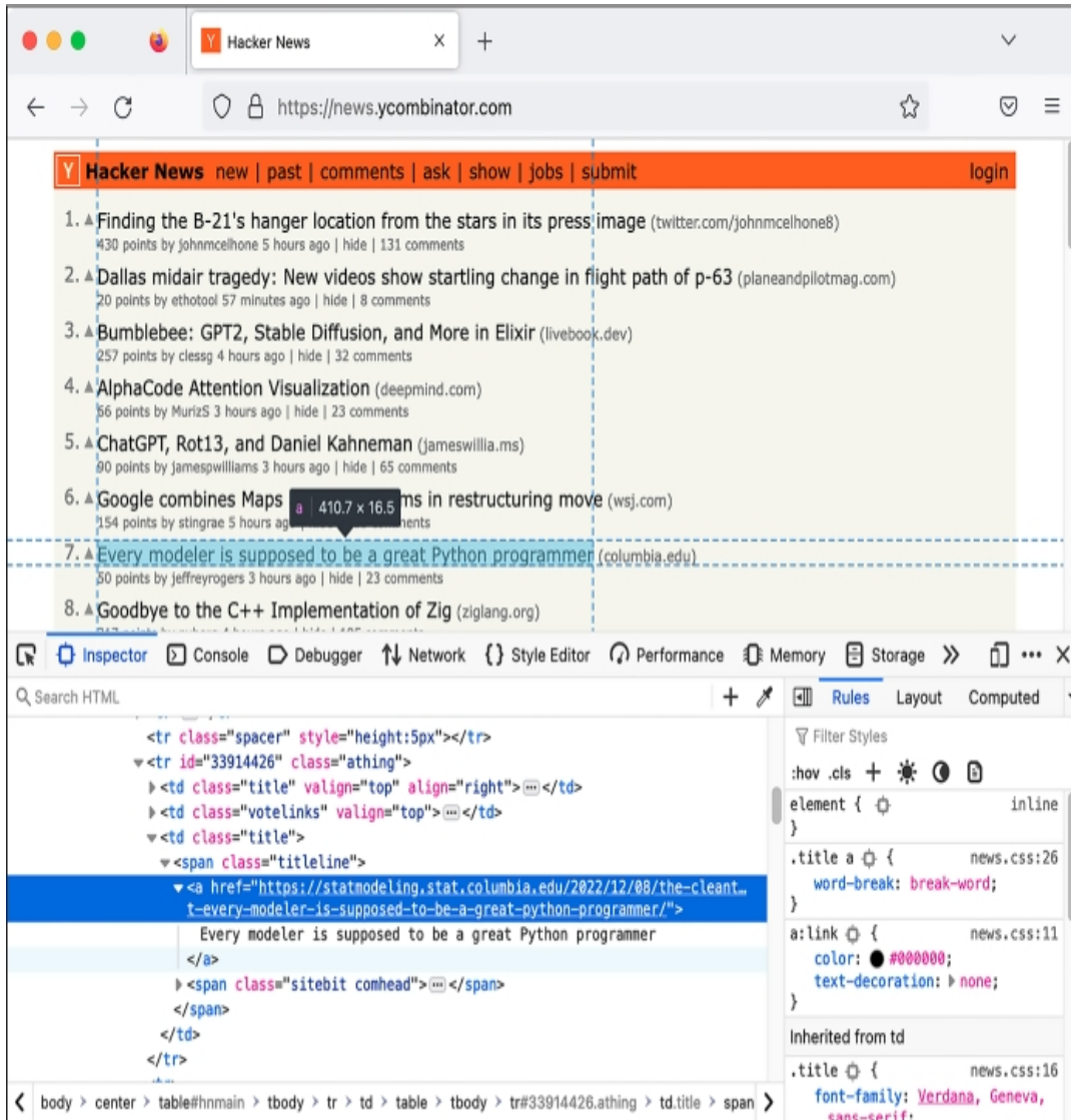
Figure B-2: Using Firefox's developer tools to inspect the HTML that makes up a Hacker News post
