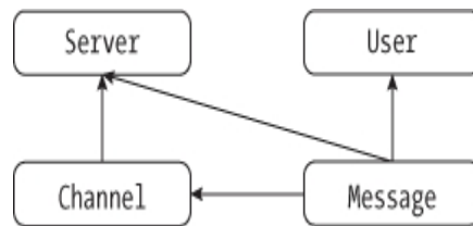
Figure 14-2: Relationships between the SQL tables in the Discord Analysis app
