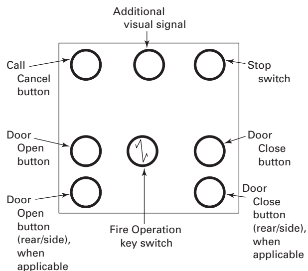
Fig. 2.27.3.3.7 Panel Layout
