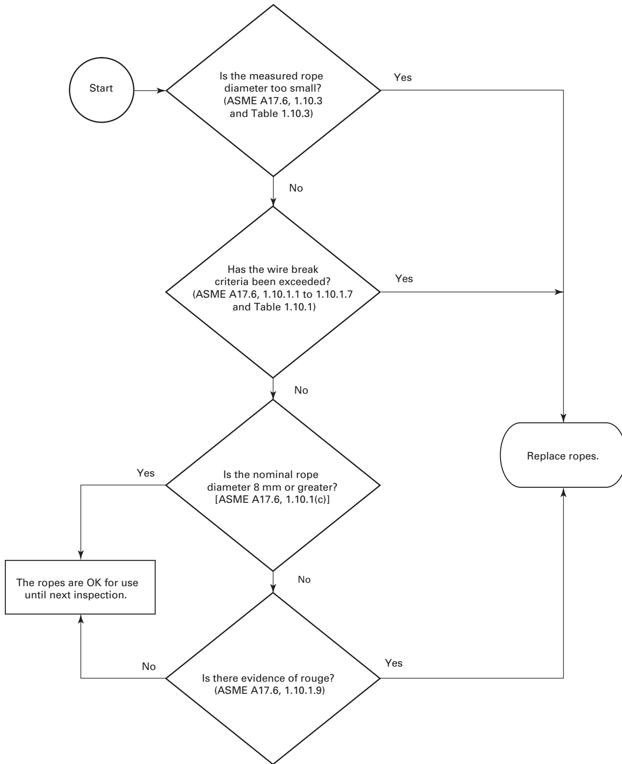
Fig. T-1 Inspection and Replacement of Steel Wire Ropes
