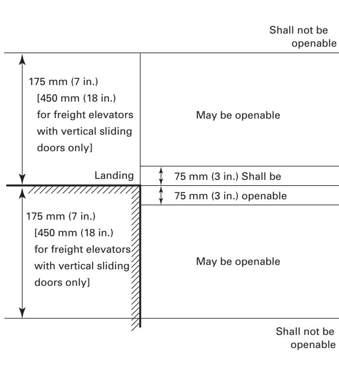
Fig. B-1 Unlocking Zone (2.14.5.7)
