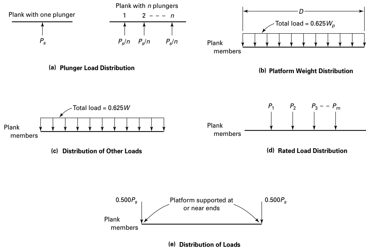
Fig. 8.2.9.1.3 Load Distribution
