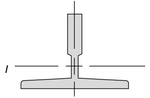
Fig. 2.23.4.1-2 Minimum Moment of Inertia About x-x Axis for a Single Guide Rail With Its Reinforcement
